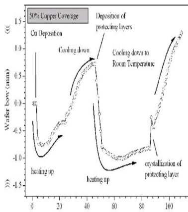
Figure 6: Evolution of the wafer bow during the simplified process flow of copper metallization in a modern power semiconductor technology.
